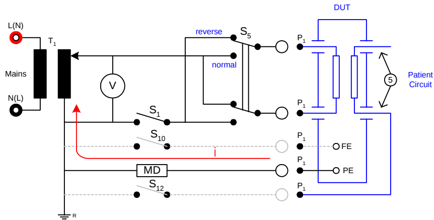
Figure 2-4a: Earth Leakage with or without Applied Part (Figure 12 of 60601-1 © IEC 2000)
